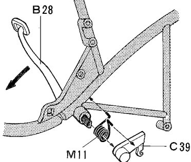
Fig. 15 Construction of Seat
