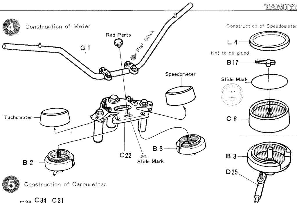
Fig. 4 Construction of Meter Firstly, assemble meter parts as illustrated below. Then, put them together as shown to the right.
