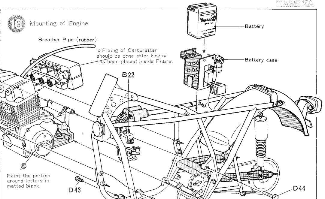
Fig. 16 Mounting of Engine Mount Engine onto Frame from the latter's right side. Next, fix Carburetter onto Engine and fasten Engine with Stopper Parts.
