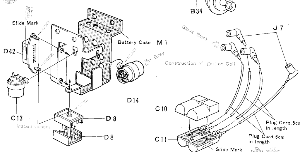
12 Construction of Electrical Parts
