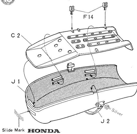
15 Construction of Seat
