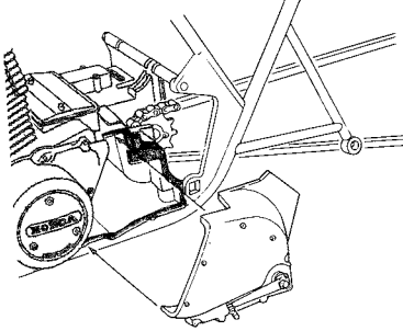
Fixing of Gear Box Cover
