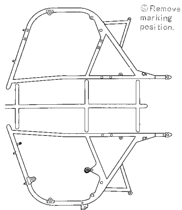
Fig. 10 Construction of Frame
