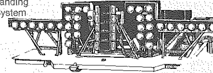
Fresnel Lens Optical Landing System
